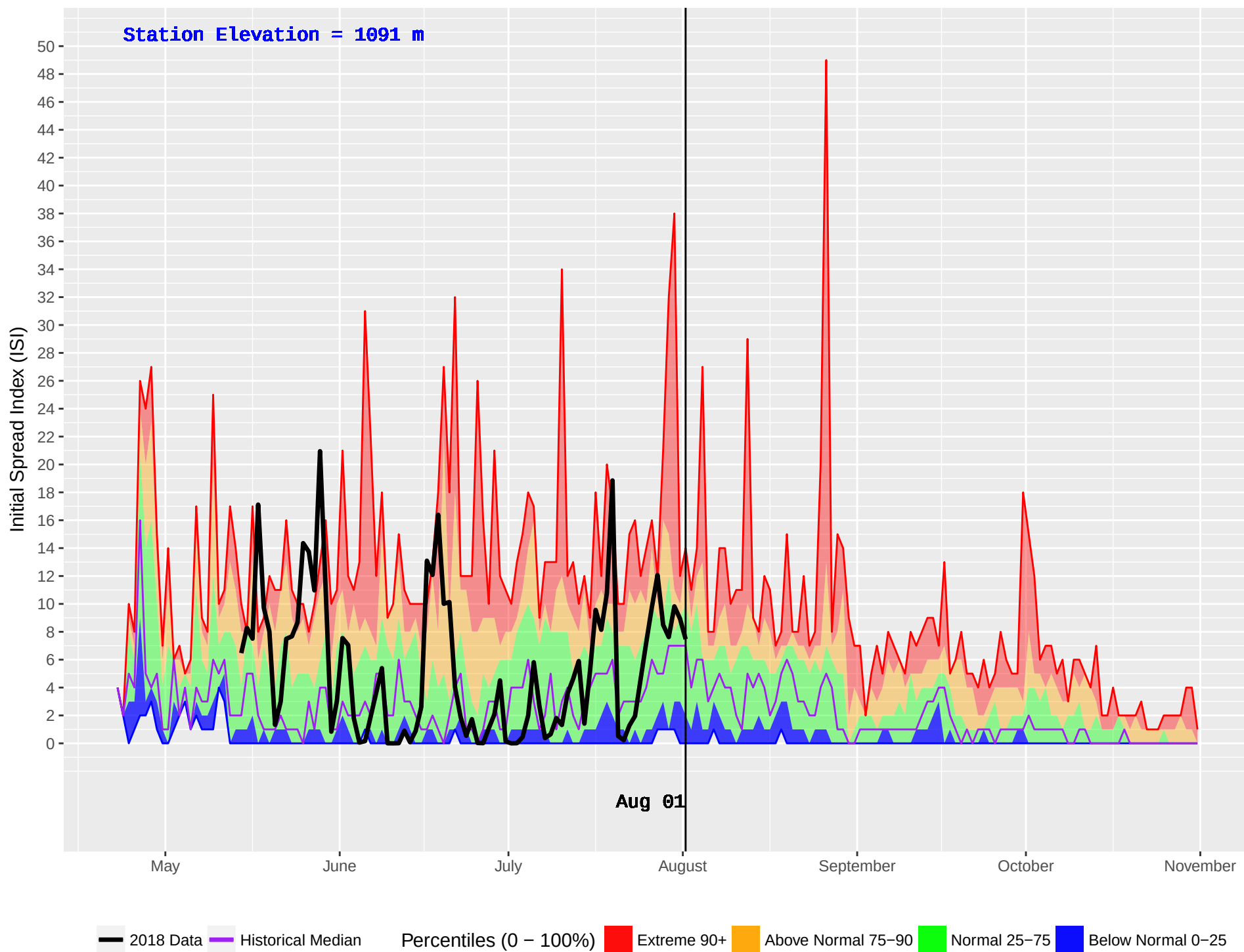
BIG MOUTH 2 (868) : Historical (2004–2016) and Current (2018) Daily Initial Spread Index (ISI)
